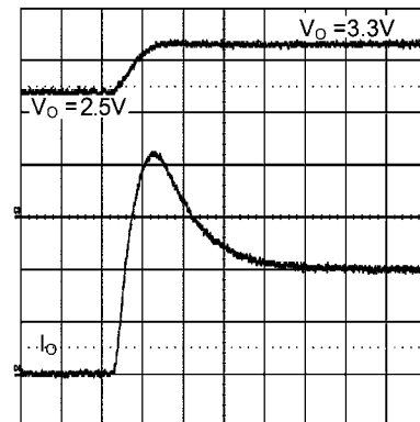
Pre-biased startup
