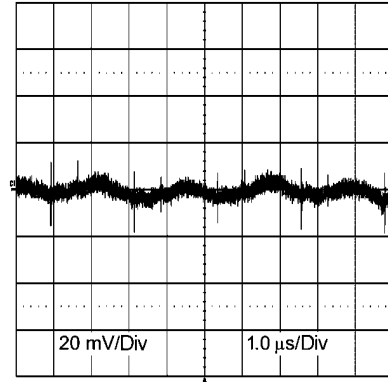
Output Ripple 12V IN 3.3V O 3A 20mV/div 1µSec/div
